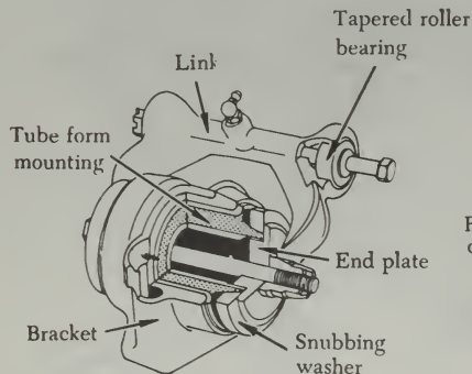
Link type dynafocal subassembly.
